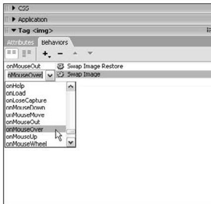
Figure 10-8: When you set up a behavior, you can specify any available action to trigger an event.
