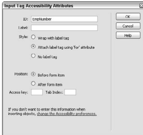
Figure 15-14: The Input Tag Accessibility Attributes dialog box.
