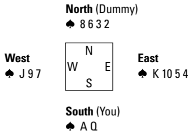
Figure 4-3: The queen can get past the king in this layout.
