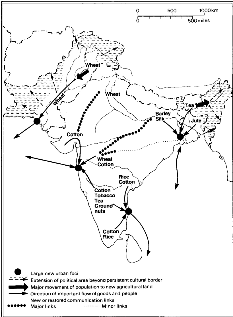
2.3 Spatial reorganisation of colonial India. The commodities indicated represent major items of the export trade in the late nineteenth century.
