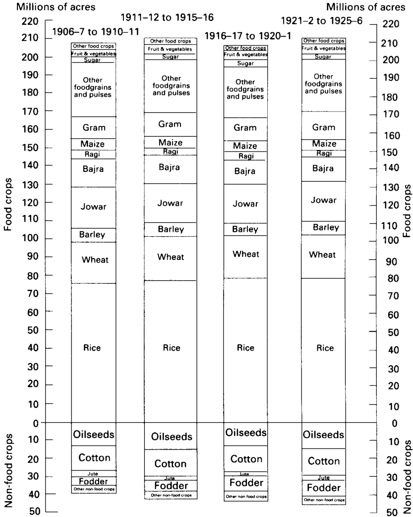
2.1 Gross area under main food and non-food crops, 1907-26
