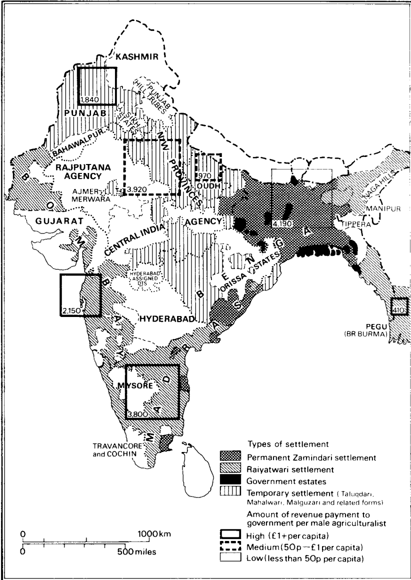
2.2 Systems of land revenue settlement. The land revenue paid by each province in the late nineteenth century is indicated by the proportional squares. The figures within each square specify the amount of payment in thousands of rupees in 1872.
