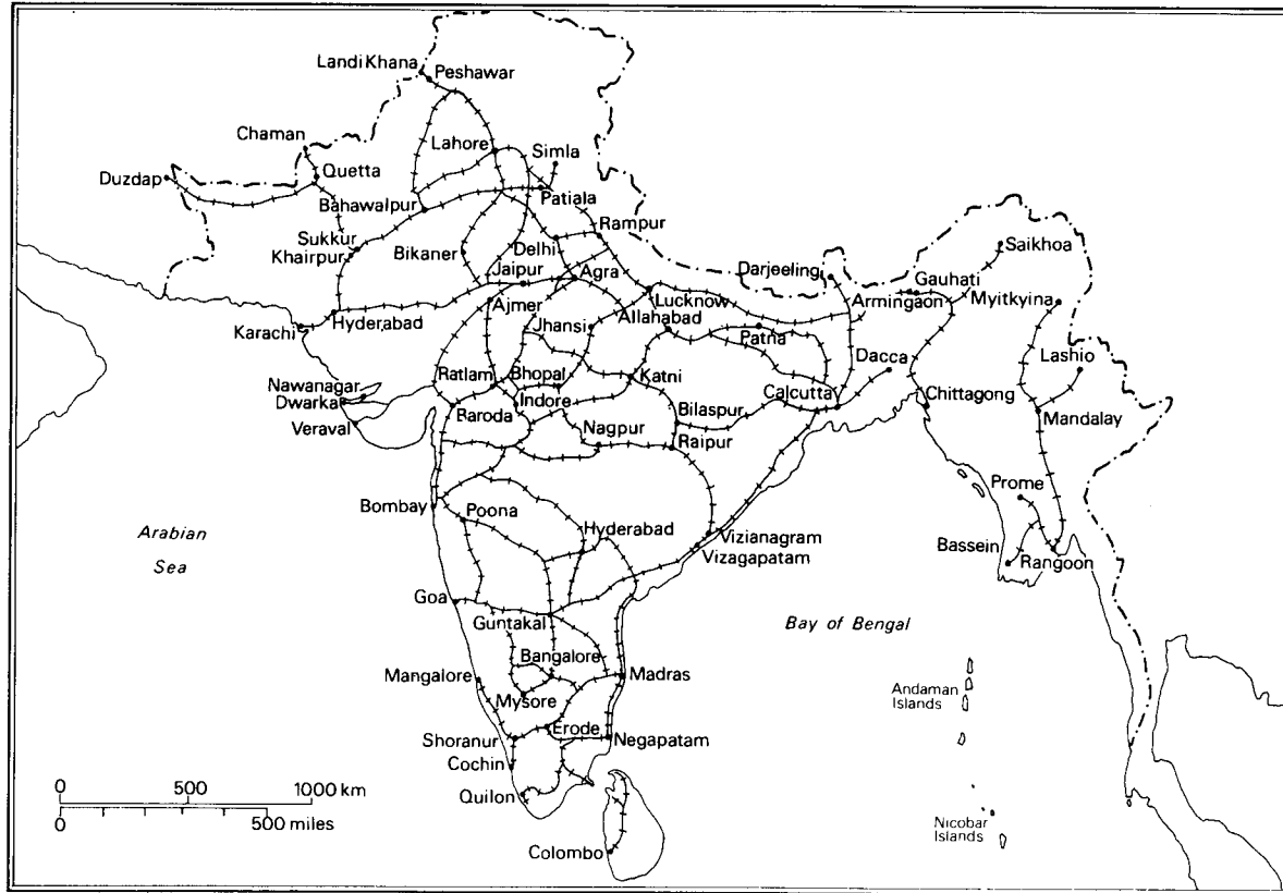
2.4 Main-line railways, c. 1947
