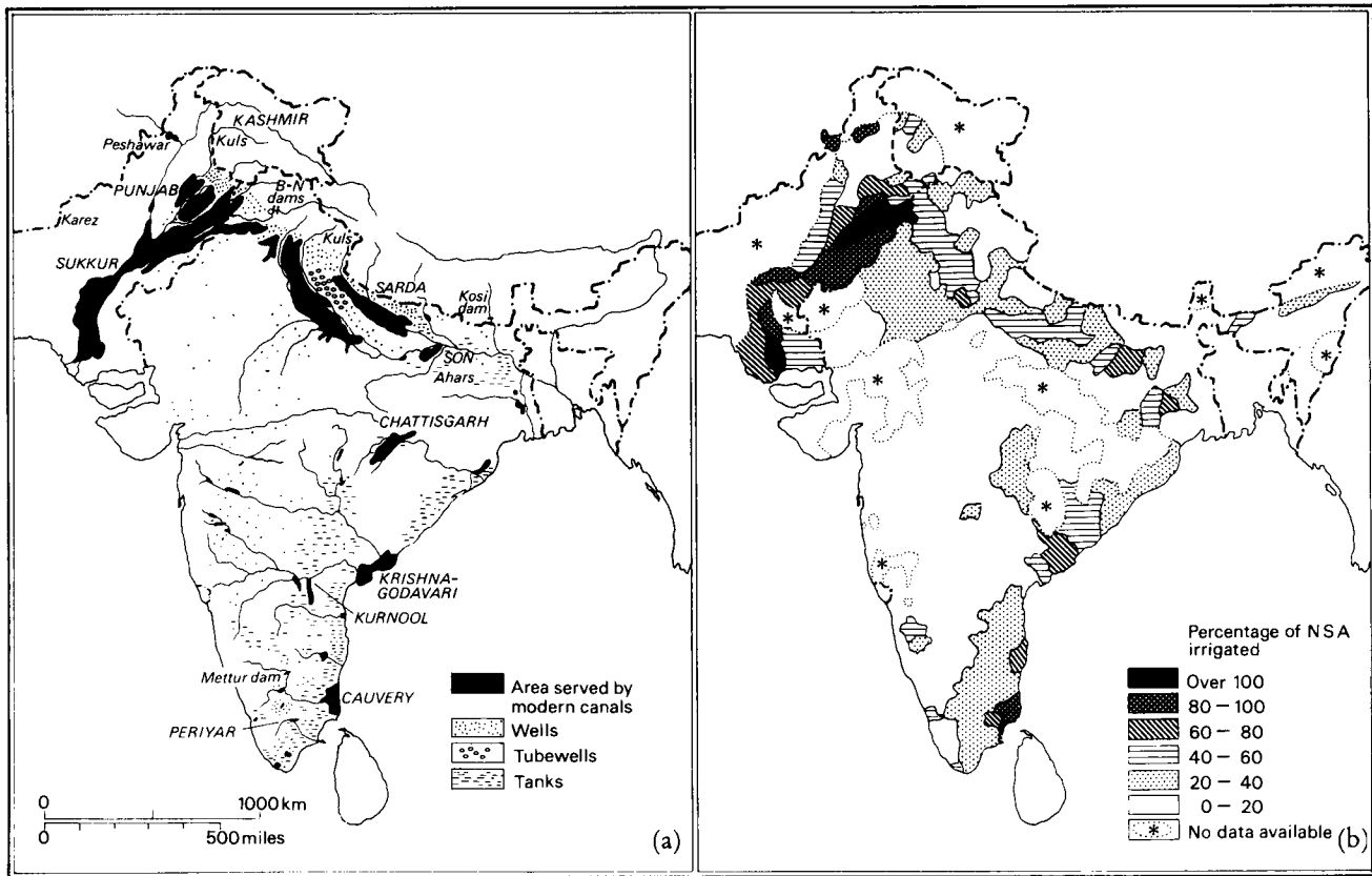
2.5(a) Types of irrigation at work in India, by district, c. 1940
