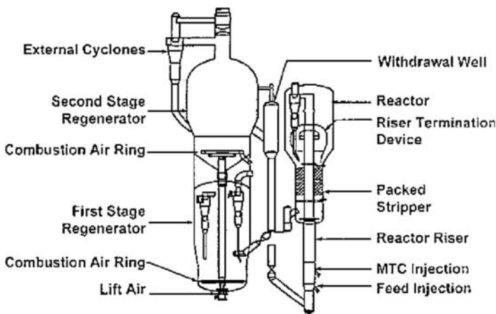
Figure 6.17. S&W/Axens R2R.
