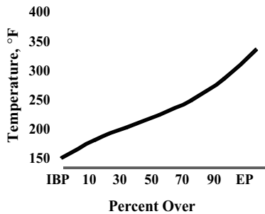
Figure 5.2. ASTM D-86 distillation curve for naphtha (1).
