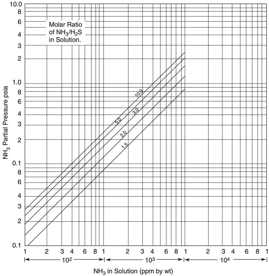
Figure 14.A.7. Partial pressure of \text{NH}_3 over aqueous solutions of \text{H}_2\text{S} and \text{NH}_3 at 210^\circ\text{F} .
