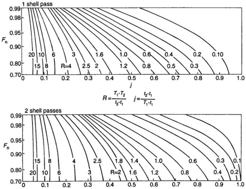
Figure 18.A.1. LMTD correction factors.
