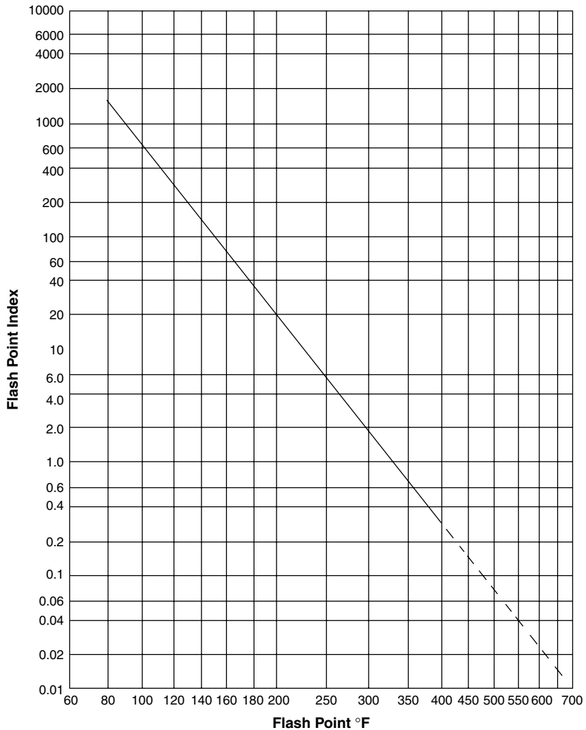
Figure 1.13. Flash point blending index.
