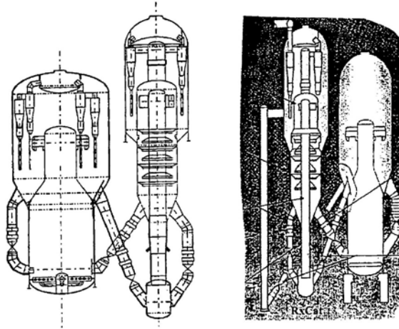
Figure 6.29. PetroFCC process.
