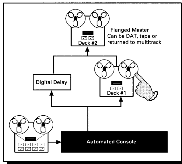
Figure 11 Modern Tape Flanging
