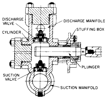
FIGURE 1 A liquid-end horizontal pump (Flowservice Corporation)
