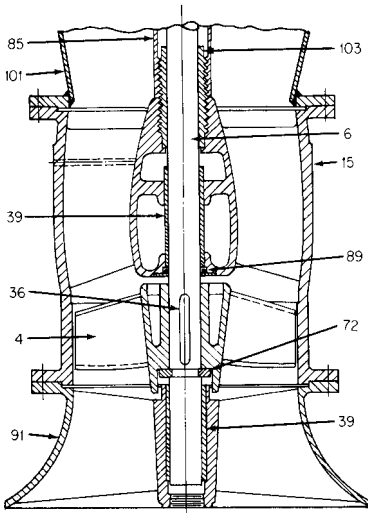
FIGURE 4 Vertical wet-pit diffuser pump bowl (the number refers to parts listed in Table 1) (Flowserve Corporation)
