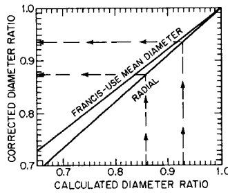
FIGURE 14 Corrections for calculated impeller diameter reductions (Reference 12)
