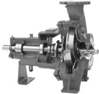
FIGURE 12 End-suction pump with semi-open impeller, inducer and renewable side plate (Flowserve Corporation)
