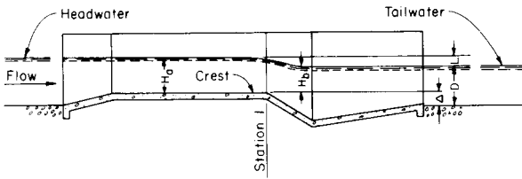
FIGURE 17 Relationships of flow depth to flume crest elevation
