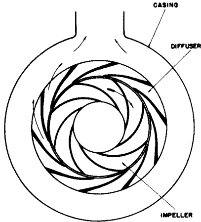
FIGURE 2 A typical diffuser-type pump
