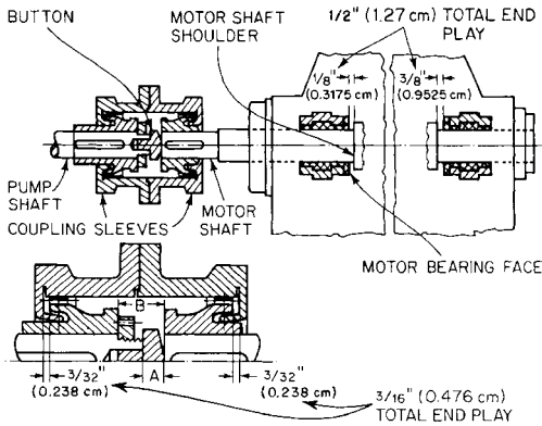
FIGURE 15 Motor-driven coupling end float limited by insertion of button between shaft end (Flowserve Corporation)
