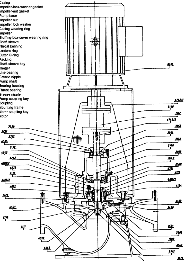
FIGURE 2 Vertical back-pull-out centrifugal pump (Flowservice Corporation)
