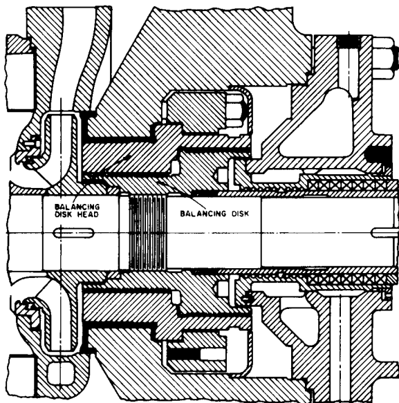
FIGURE 64 A combination balancing disk and drum with a disk located in the center portion of the drum (Flowsolve Corporation)
