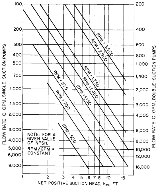
FIGURE 23 Capacity (flow rate) and speed limitations for condensate pumps with shaft through eye of impeller ( \text{ft} \times 0.3048 = \text{m} ; \text{gpm} \times 0.06309 = \text{l/s} ) (adapted from Hydraulic Institute ANSI/HI 2000 Edition Pump Standards, Reference 27)
