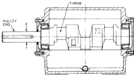
FIGURE 16 A cast crankshaft (Flowserve Corporation)
