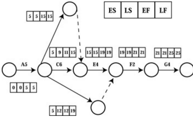
Figure 3-7: Project activities CPM
