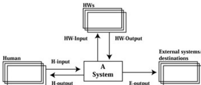
Figure 18-7: A sample context diagram
