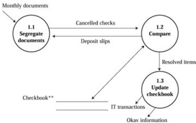
Figure 18–11: A sample of level 2 partitioning
