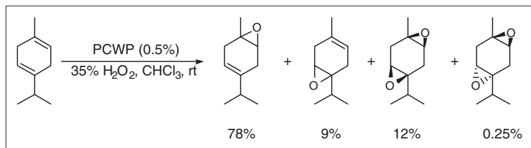
Scheme 10.60
