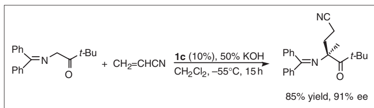
Scheme 10.35
