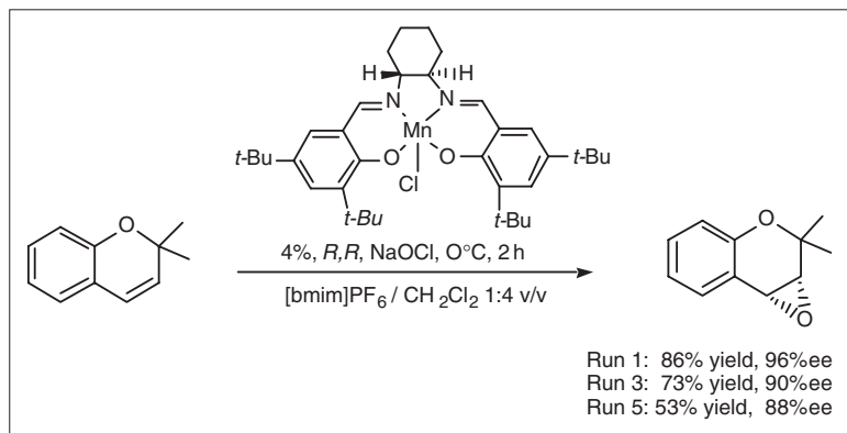
Scheme 10.72
