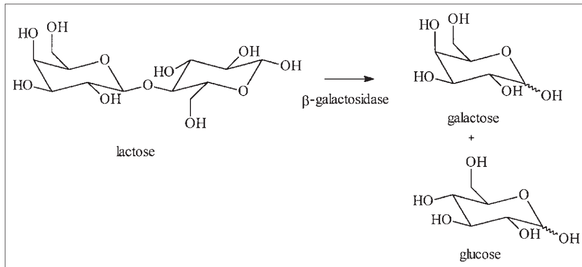
Fig. 9.4 Conversion of lactose to glucose and galactose by \beta -galactosidase.
