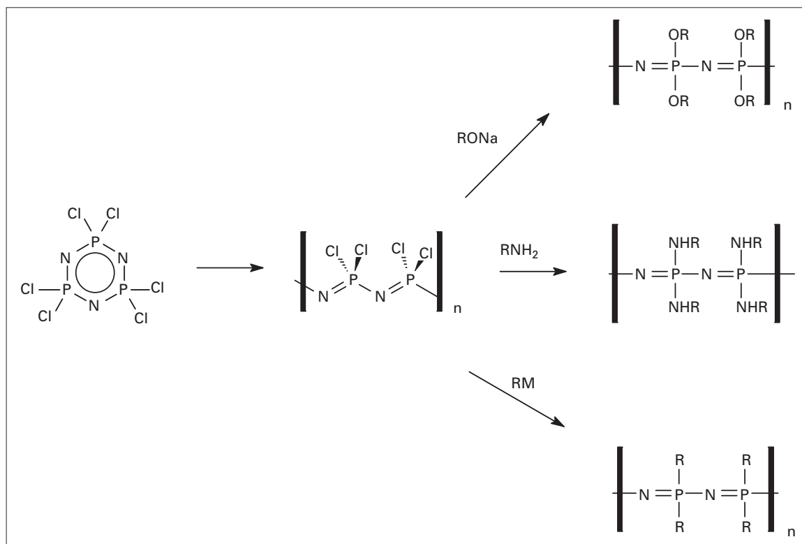
Fig. 8.16 Polyphosphazenes.
