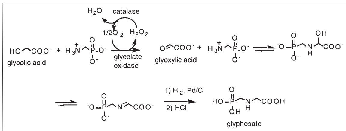
Scheme 14.20
