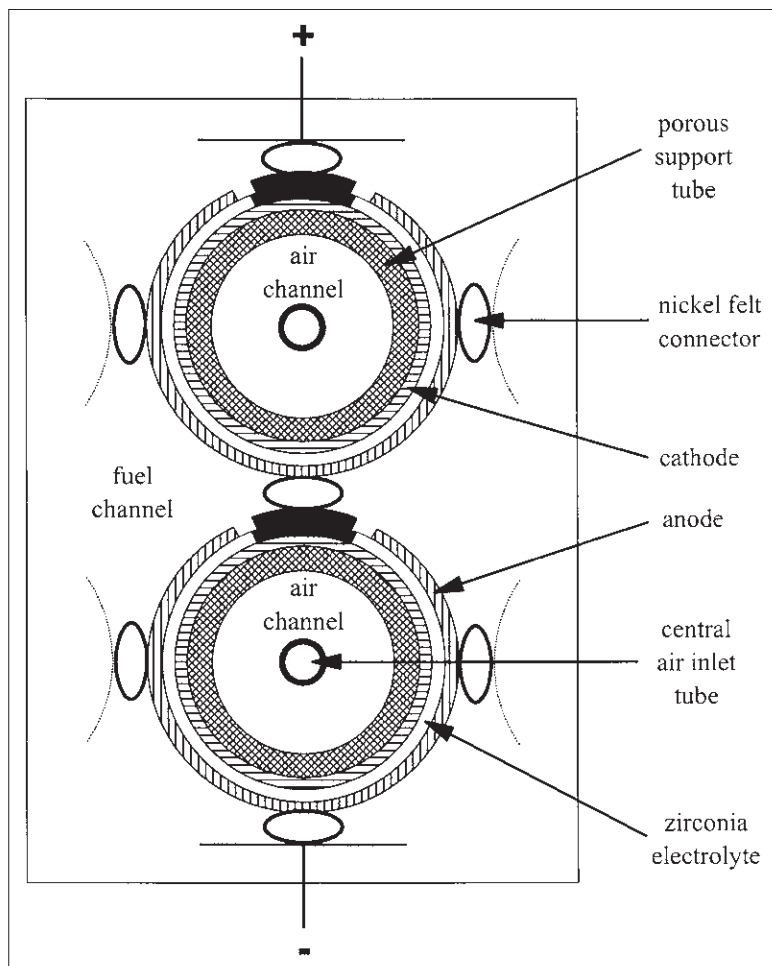
Fig. 20.5 Schematic diagram of a tubular solid oxide fuel cell (not to scale): Siemens Westinghouse design, plan view.
