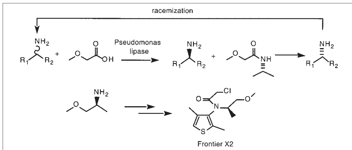
Scheme 14.21
