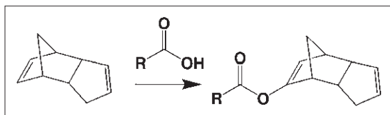
Scheme 6.26
