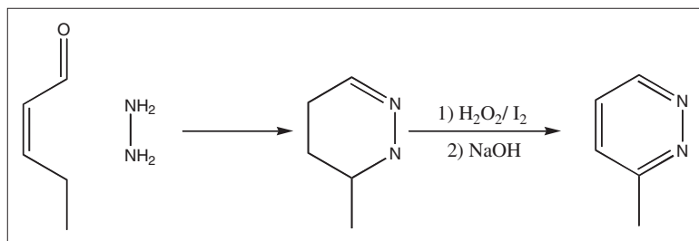
Fig. 11.39 Aromatisation of a heterocyclic intermediate.
