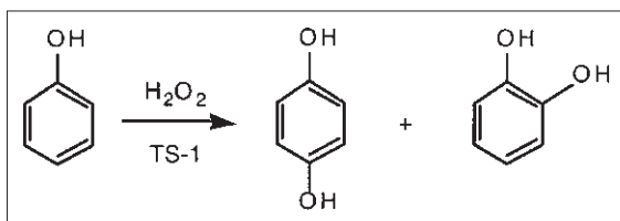
Scheme 14.2
