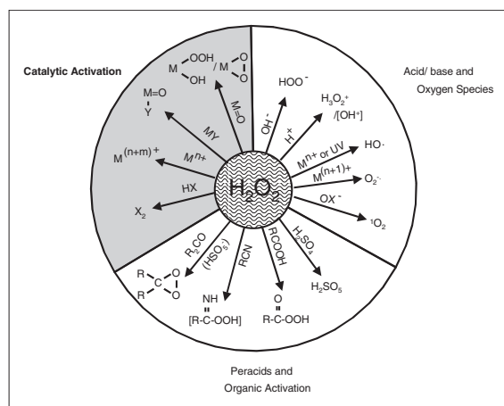
Fig. 11.3 Activation of hydrogen peroxide.
