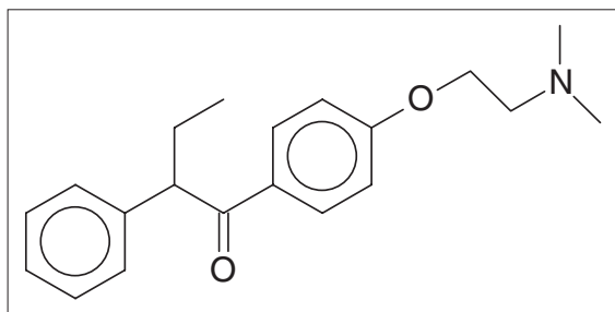
Scheme 13.26
