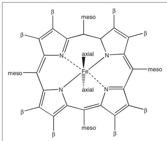
Fig. 11.8 Metalloporphyrin structure.
