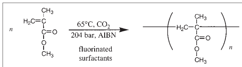
Scheme 21.4 Synthesis of poly(methyl methacrylate) via dispersion polymerisation in sc\text{CO}_2 .
