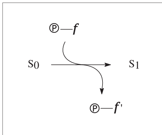
Fig. 8.1 Polymer-supported reagents.
