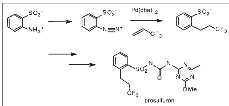
Scheme 14.18
