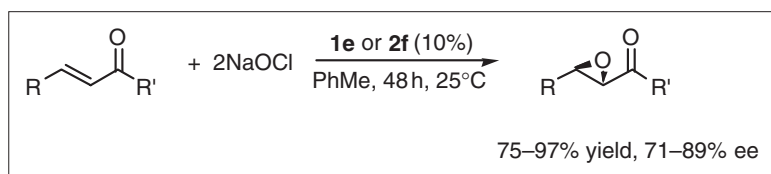
Scheme 10.37
