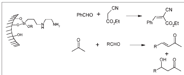
Fig. 7.35 Reactions catalysed by a diamino-micelle-templated silica.
