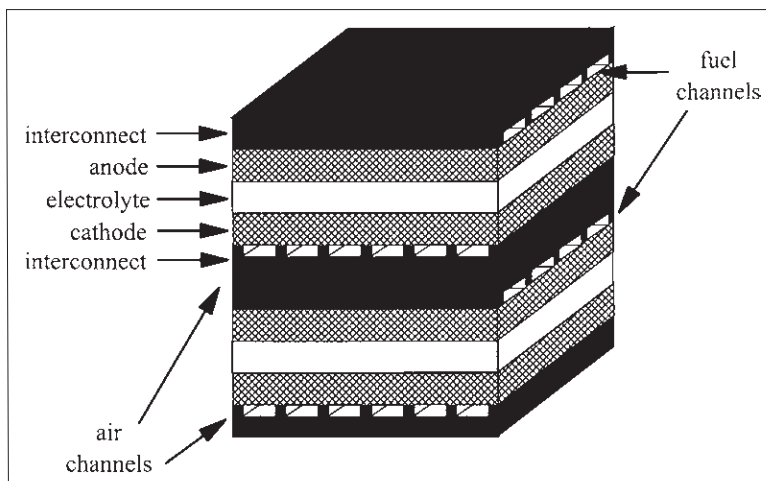
Fig. 20.6 Schematic diagram of a planar solid oxide fuel cell stack (two cells, not to scale).
