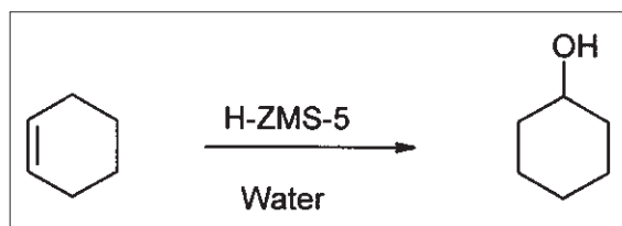
Fig. 2.18 Asahi route to cyclohexanol.
