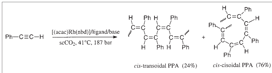
Scheme 21.5 Rhodium-catalysed synthesis of poly(phenylacetylene)(PPA) in sc\text{CO}_2 .
