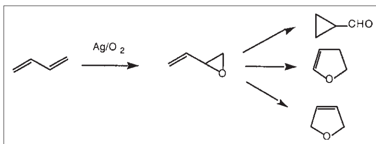
Scheme 14.5
