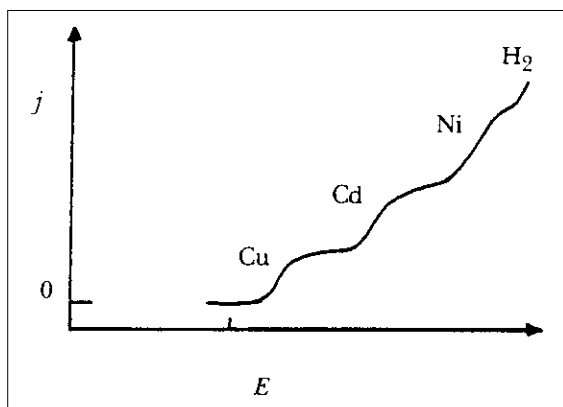
Fig. 19.16 Schematic diagram of polarisation curves for multi-deposition reactions.
