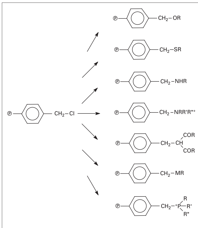
Fig. 8.7 Chemical derivatisations of chloromethylated polystyrene.
