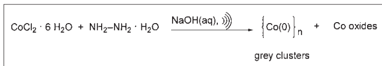
Scheme 16.16 Sonochemical formation of cobalt nanoclusters.
