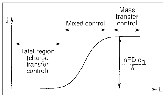
Fig. 19.2 Schematic representation of the overpotential–current density relationship.
