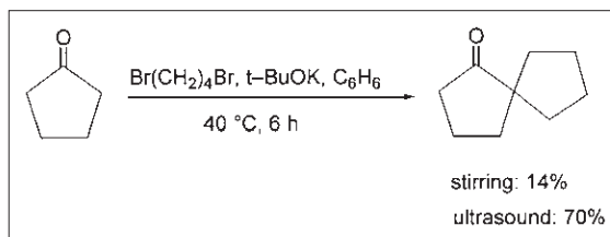
Scheme 16.11 Synthesis of spiroketones from cycloalkanones.
