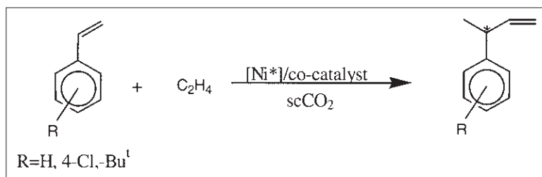
Scheme 21.6 Hydrovinylation of styrenes in sc\text{CO}_2 .
