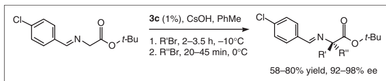
Scheme 10.41
