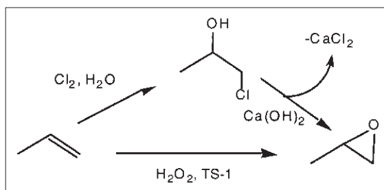
Scheme 14.3
