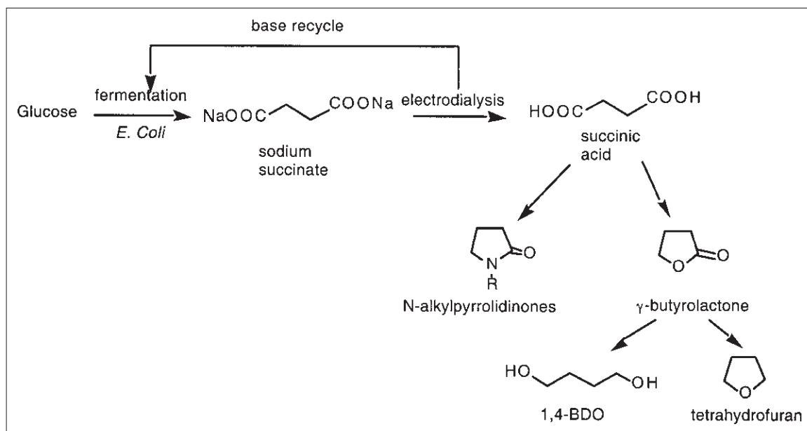
Scheme 14.22
