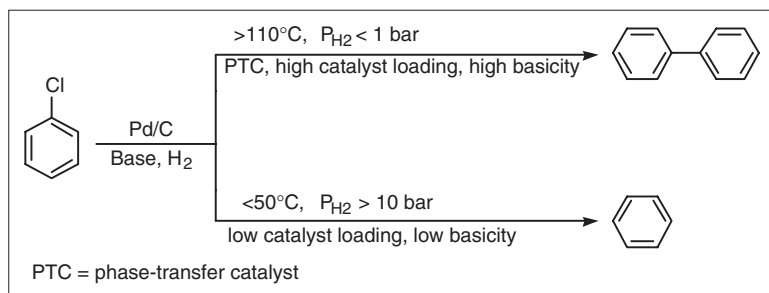
Scheme 10.52
