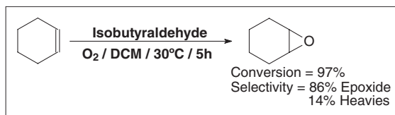
Scheme 13.32
