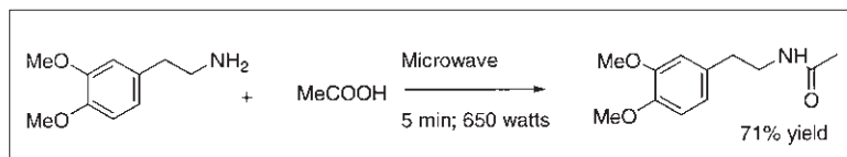
Scheme 17.2 Direct amidation [48].
