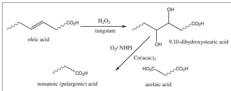
Fig. 11.23 Oxidative cleavage of oleic acid using hydrogen peroxide and oxygen.
