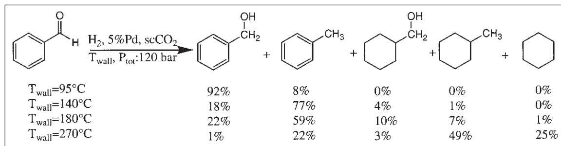
Scheme 21.14 Hydrogenation of benzaldehyde in \text{scCO}_2 .
