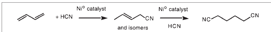
Scheme 14.7
