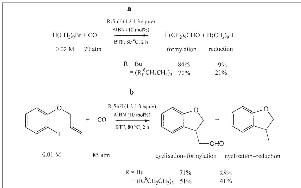
Fig. 22.14 Comparison of the reactivity of tributyltin hydride and the fluorous analogue in (a) formylation and (b) cyclisation-formylation reactions.
