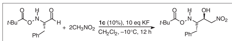
Scheme 10.36
