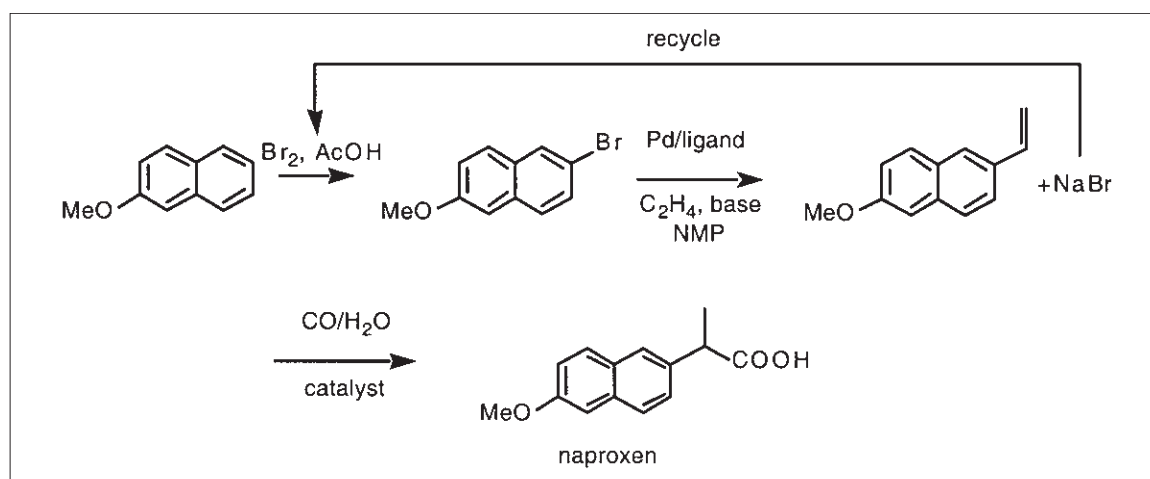
Scheme 14.17
