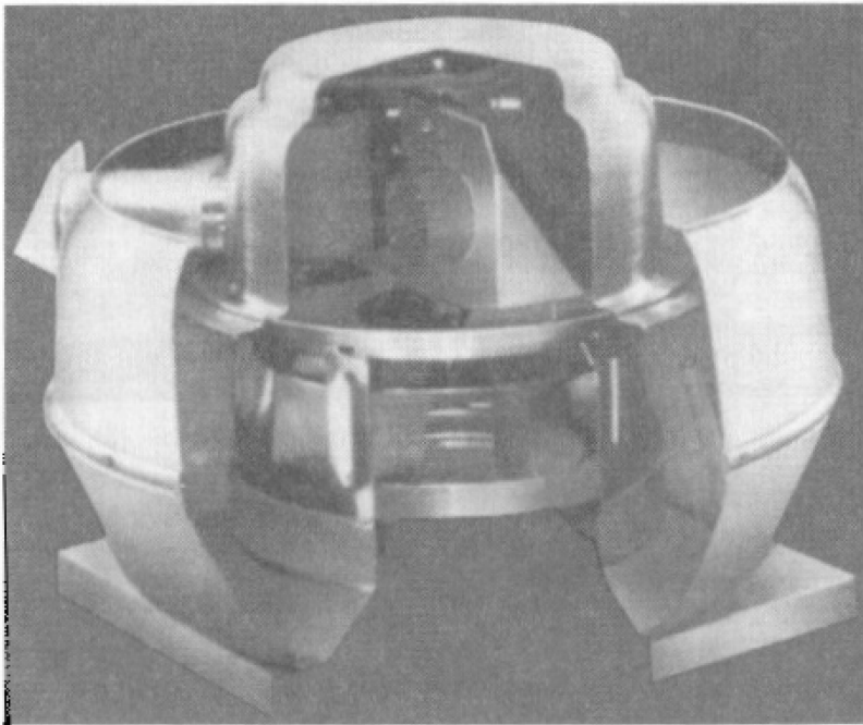
FIGURE 10.3 Exhaust roof ventilator, upblast, with a centrifugal fan wheel and belt drive. (Courtesy of FloAire, Inc., Bensalem, Pa.)
