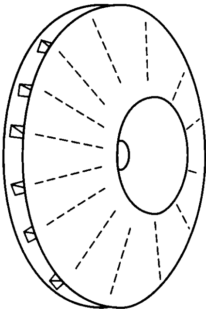
FIGURE 7.32 Turbo blower wheel with a diameter ratio of 0.50 and with 14 radial blades 1\frac{1}{4} to 1 in wide. Each blade has a bent-over strip for riveting to the back plate and little tabs that fit into slots in the shroud for fastening.
