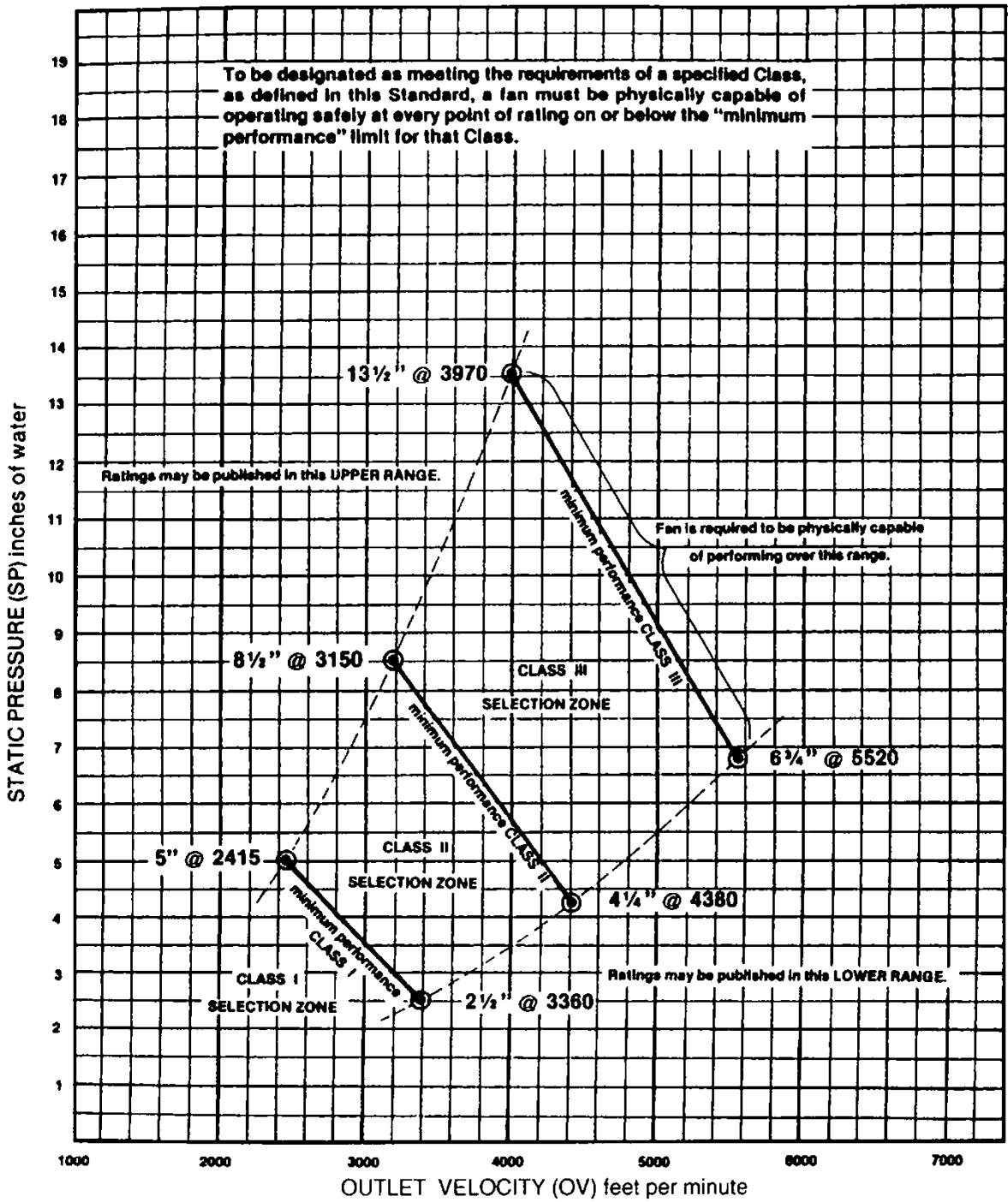
FIGURE 23.8 Operating limits for double-width centrifugal fans with airfoil or backwardly inclined blades per AMCA Standard 99-86.
