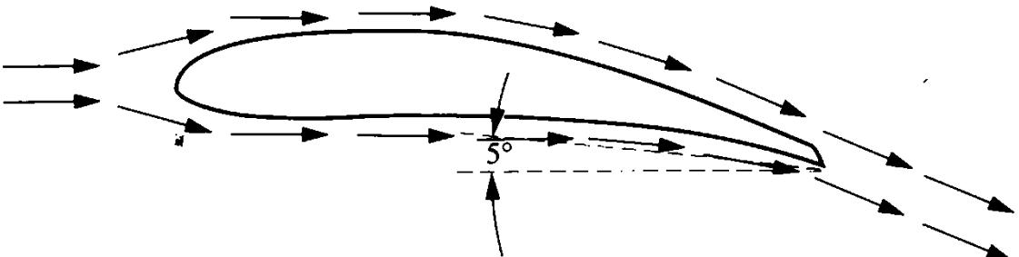
FIGURE 2.6 At a 5^\circ angle of attack, the airflow is smooth and follows the contours of the airfoil. The direction of the airflow is deflected by 13.5^\circ .
