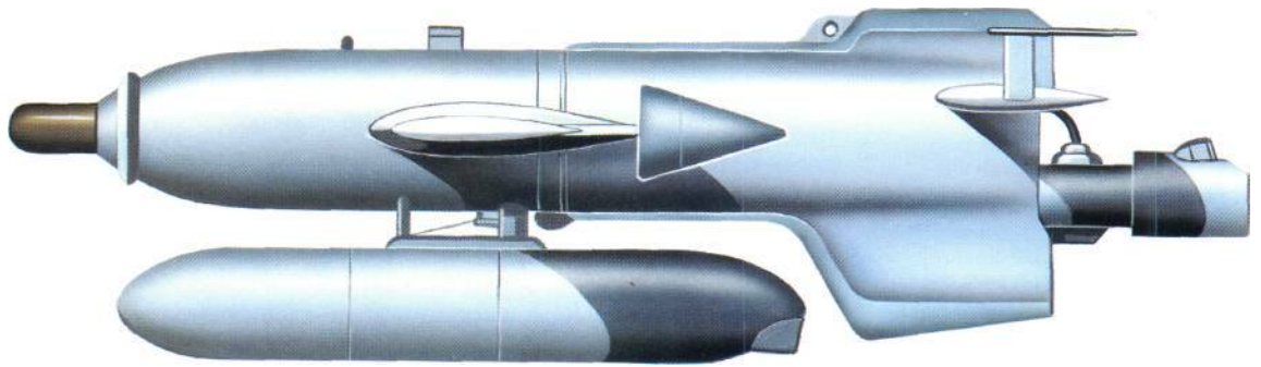
The Henschel Hs 293A stand-off guided bomb was dropped from the carrier aircraft on a parallel course to the target on the port side, and radio-guided to the target. A flare in the rear of the bomb gave visible evidence of the missile's position to the aimer.
