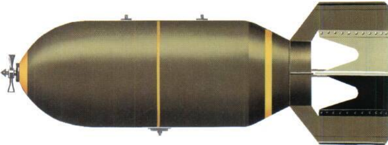
A typical general purpose bomb in use with US forces was the 227-kg (500-lb) weapon shown. It had an explosive filling to weight ratio of 51 per cent brought about by the use of a thin case. The bomb had two fuses, one in the nose and the other in the tail.
