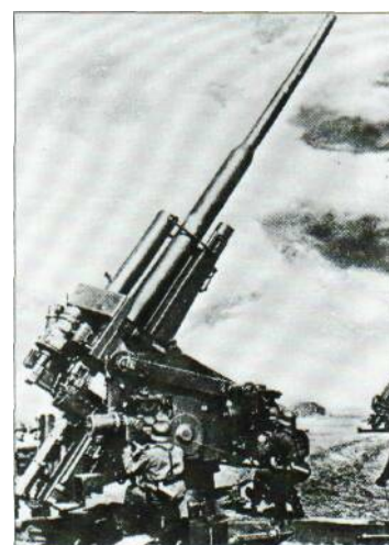
This photograph of 12.8-cm Flak 40s in the field was taken in 1940 in order to show the 'might' of the German army's anti-aircraft field defences. In fact only one battery was so used before all production of the gun was switched to the home defence of the Reich. This one battery was also moved out of the field.
