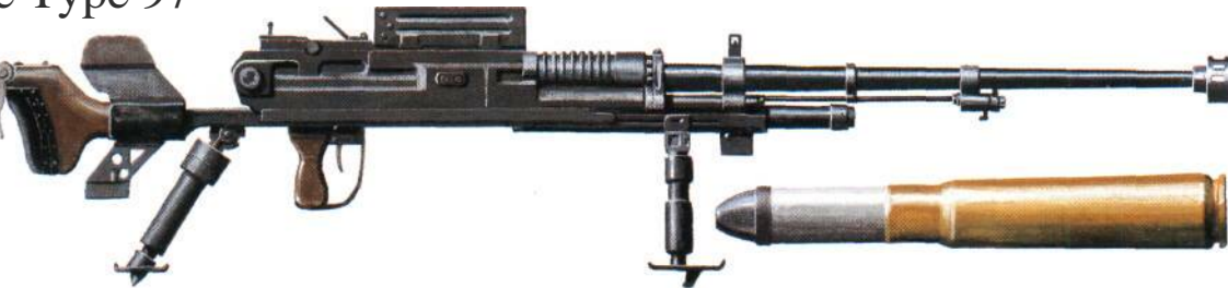
The Japanese Type 97 anti-tank rifle was a heavy weapon that weighed 51.75 kg in action, mainly due to the gas-operated semi-automatic mechanism. It had a calibre of 20 mm (0.787 in) and required a crew of two men to fire and four to carry it, using a system of frames.
