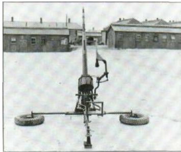
Above: Broken down into its operating position, a Polsten gun shows the sparse construction of this simplified, lightened version of the well-tried Oerlikon.
