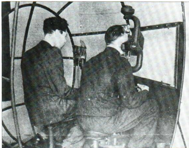
Crew members learn to control the Henschel Hs 293 guided bomb in a simulator. The guidance operators always sat on the starboard (right) side of the cabin, and therefore it was always necessary to attack a target from the port side and in the same movement direction.
