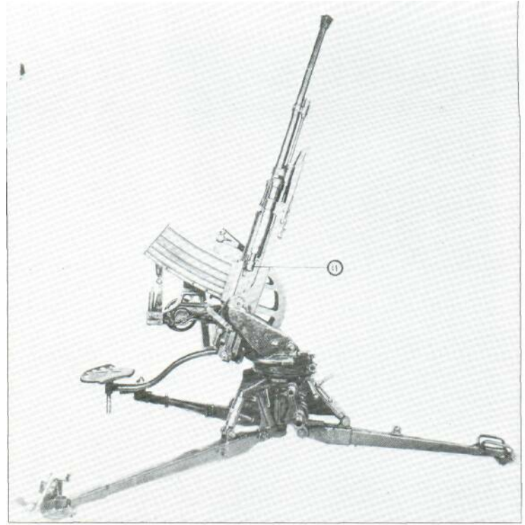
This Type 98 is emplaced for the anti-aircraft role and has the barrel at a full elevation. The 20-round box magazine is fitted, and here the figure 11 points to a cocking handle.
