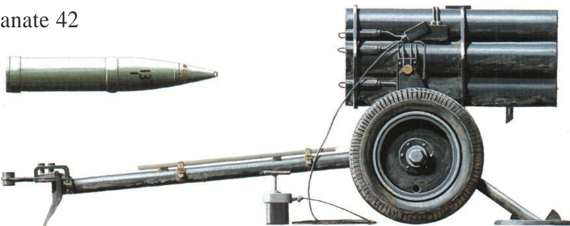
The 21-cm rocket superficially resembled a conventional artillery round, but its streamlined nose was hollow and its base had 22 angled venturi to produce spin stabilization.
