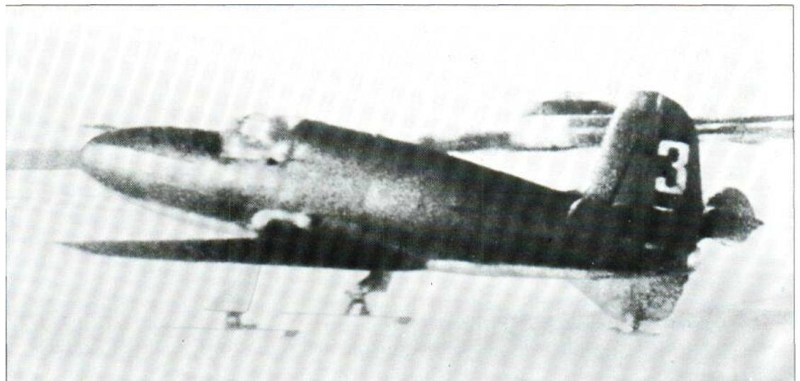
Above: The third prototype BI was fitted with retractable skis which could be interchanged with wheels depending on the ground conditions. Armament was two 20-mm cannon.
