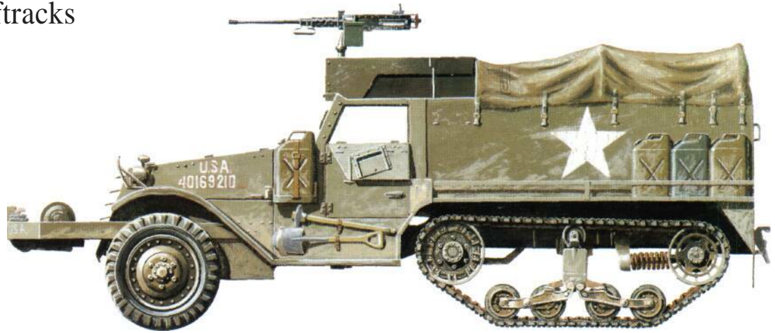
Above: The American M3 halftrack was such a widely used vehicle that it became a virtual trademark of the US Army and other Allied forces, including the Red Army. This M3 is complete with the canvas tilt, a forward-mounted winch and the 'pulpit' machine-gun mounting, here with a 0.50-in (12.7-mm) Browning.
