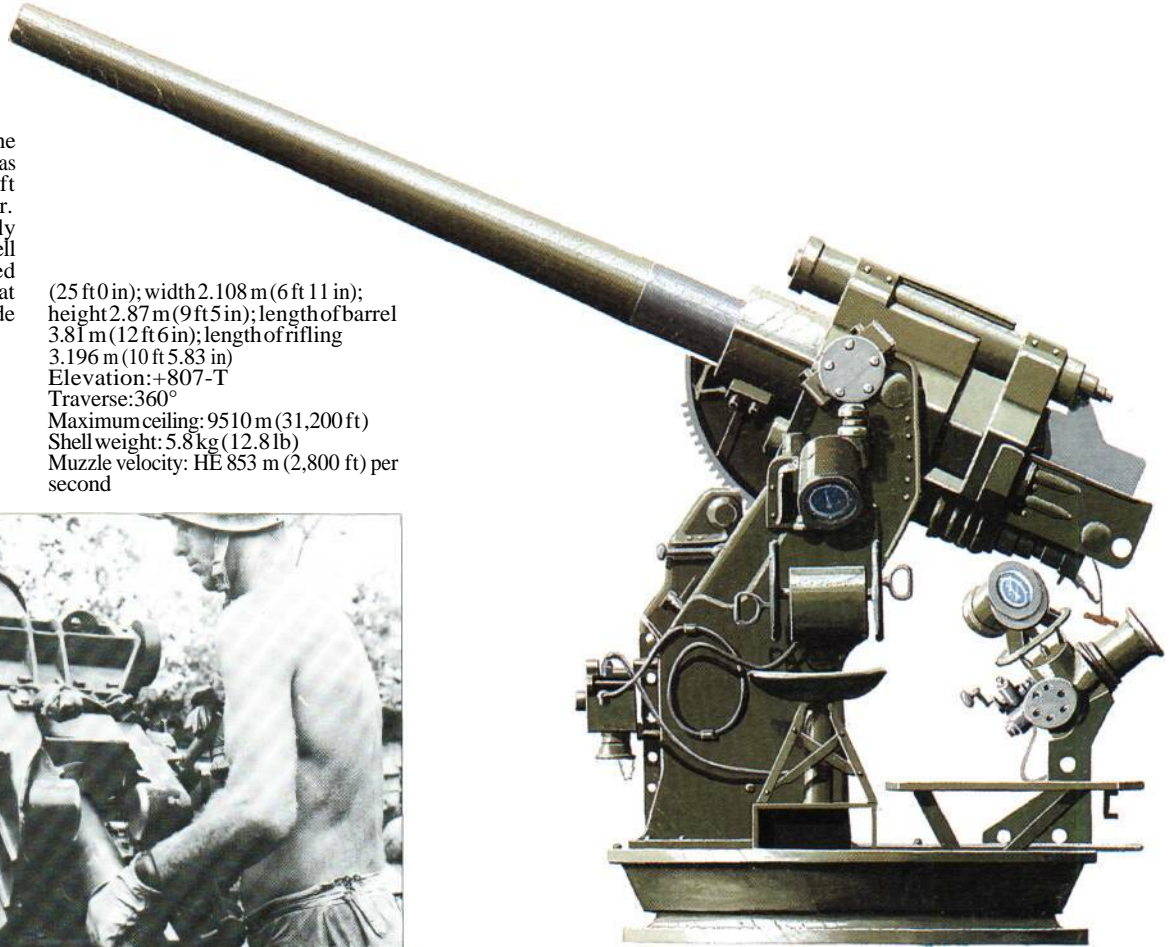
Above: In 1941 the American 3-in (76.2-mm) gun was still in service in several forms. This static version was the 3-in Gun M4 on Mount M3, and was used in such locations as the Philippines and the Canal Zone.
