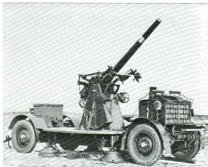
The usual model of the 3-in (76.2-mm) gun in use with the BEF in 1940 was this platform version, complete with twin axles. The platform used
