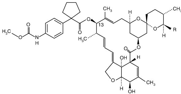
Latidectin
