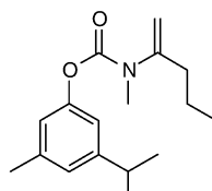
promacyl
