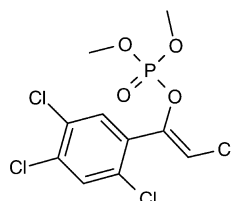
tetrachlorvinphos (CVMP)
