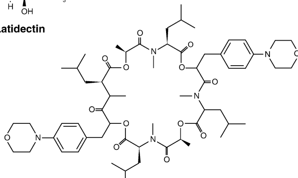
Emodepside
