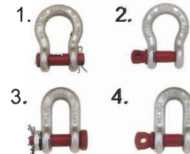
High tensile steel shackles. To obtain this high strength, after forging the shackles are subjected to heat treatment. (Quenched and Tempered)
