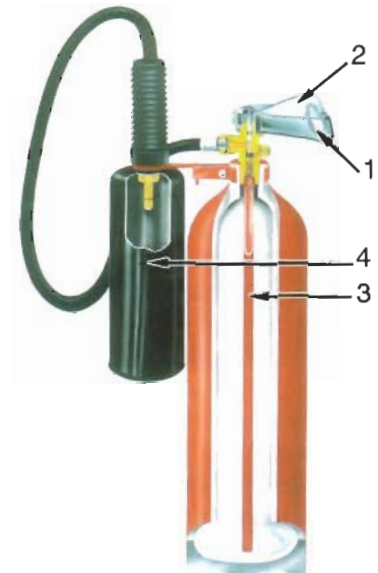
Cross-section of CO 2 -extinguisher
