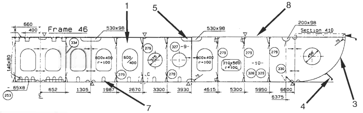
Tansverse cross-section
