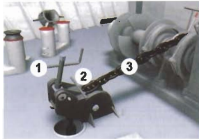
Chain stopper with tensioner
