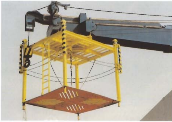
At the end of the pallet-swinger is a (yellow) pallet-cage
