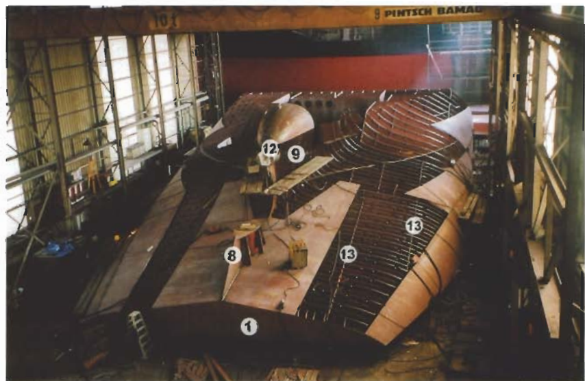
Construction of part of the aft ship of a container feeder
