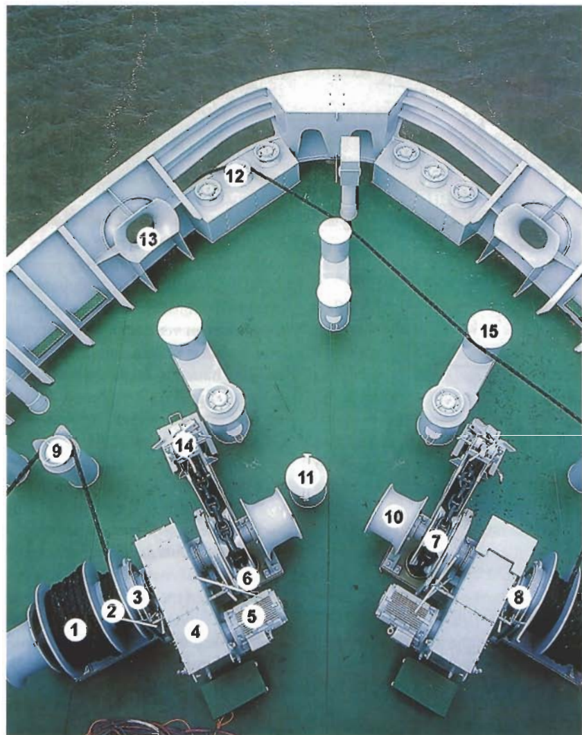
Foreccastle deck
