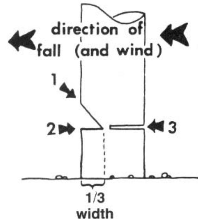
Chainsaw felling; note sequence of cuts.
